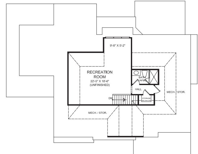
THIRD FLOOR
